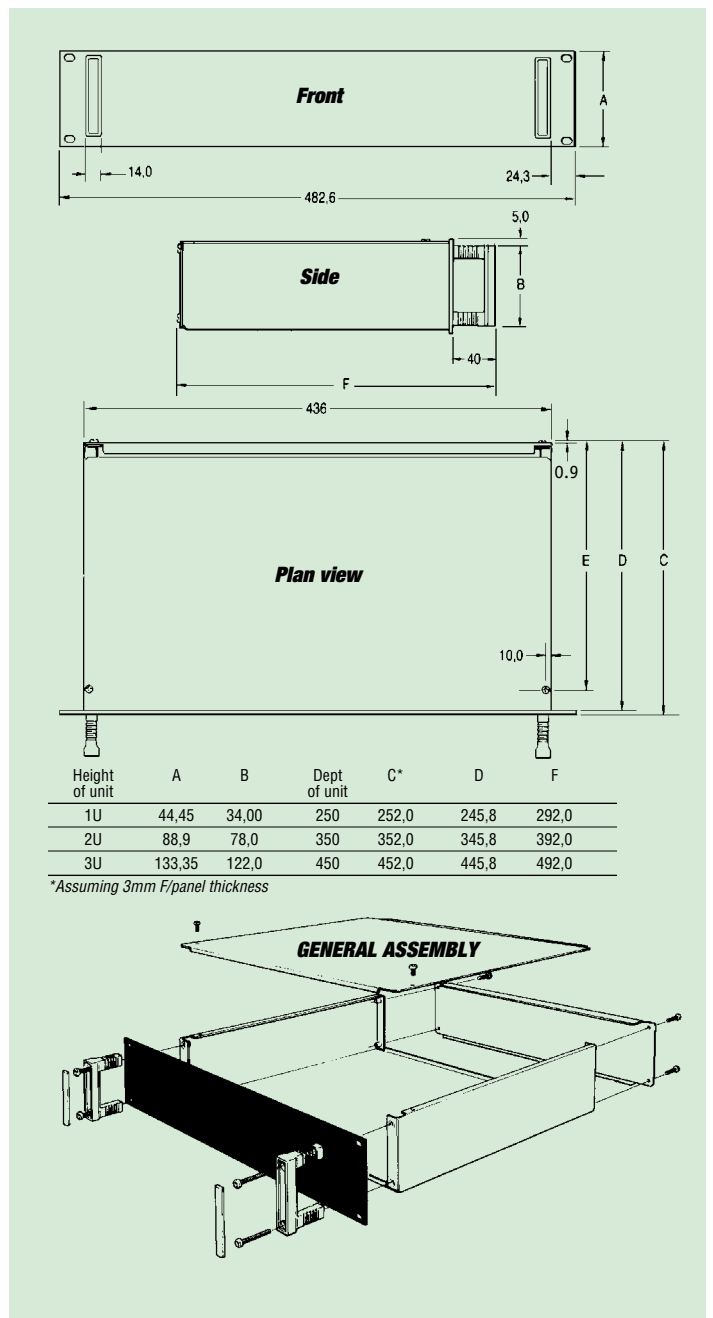
19" RACK CASES
